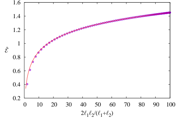
FIG. 5. Upper bound against CFT scaling variable with \ell_1 + \ell_2 = 200 fixed and varying \ell_1 . For comparison, the solid line shows the equal-segment result (116), with \ell_1 = \ell_2 = \ell .
