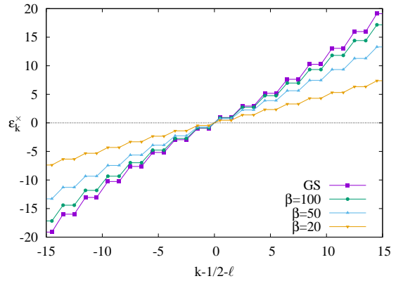
FIG. 6. Thermal single-particle spectra for \ell = 100 and various \beta .
