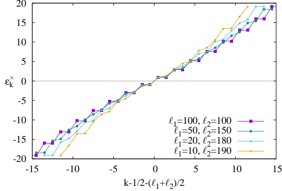
FIG. 4. Single-particle spectra \varepsilon_k^\times for \ell_1 + \ell_2 = 200 and various \ell_1 .
