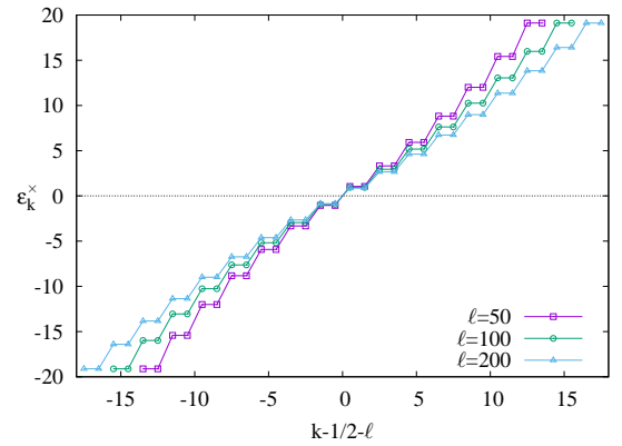
FIG. 3. Single-particle spectra \varepsilon_k^{\times} for various \ell .
