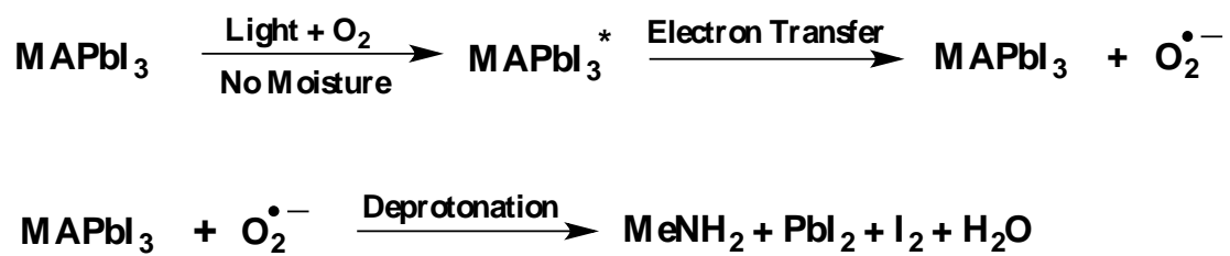
Figure 6. Reaction scheme indicating a potential route for degradation caused by superoxide as predicted from the obtained data reported. The \text{MAPbI}_3^* intermediate indicates photo-excitation and the formation of the photo-generated electron that is subsequently transferred to oxygen.
