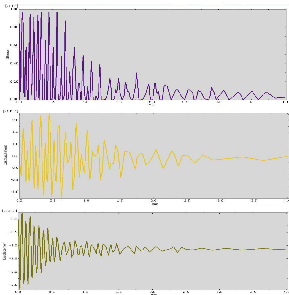
Figure 5. The time history of stress in dam heel, horizontal and vertical crest displacement under Kobe earthquake
