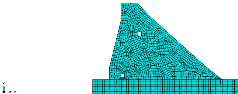
Figure 3. Meshing by finite element analysis of Zavin concrete gravity dam
