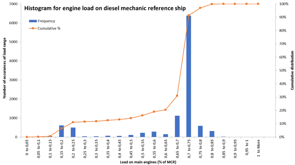
Fig. 7 Case study vessel load spectrum
