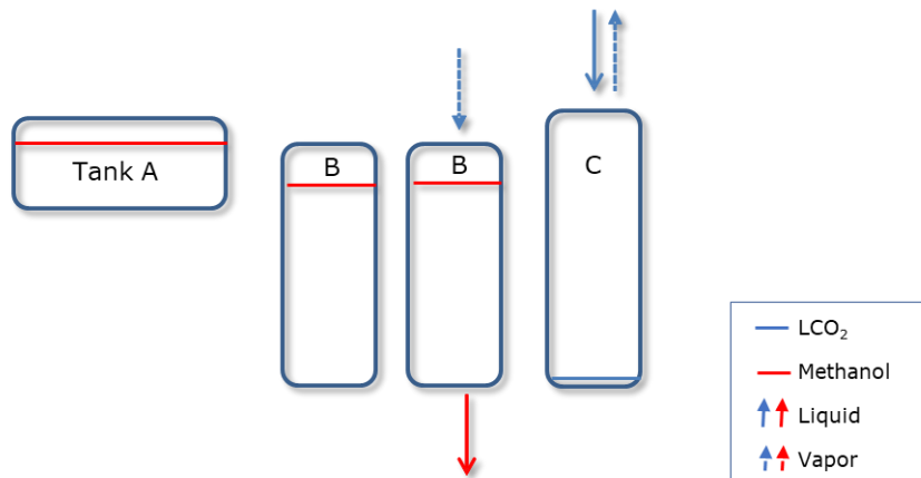
Fig. 5 Combined methanol / CO 2 tank system
