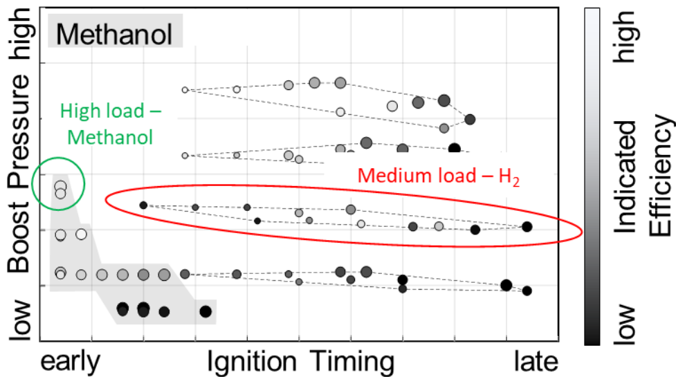
Fig. 4 Operating ranges and transition between methanol and hydrogen operation
