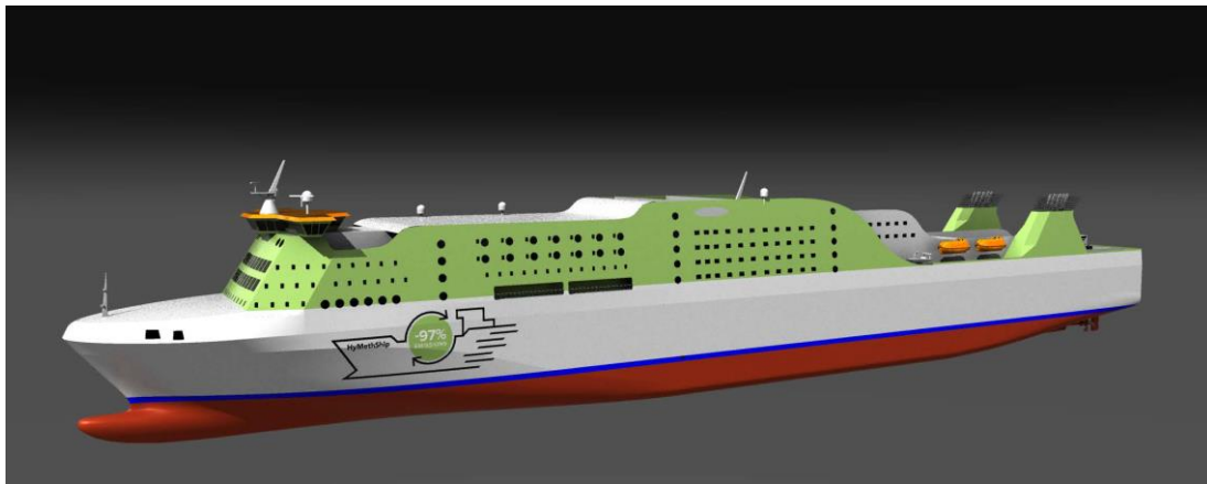
Fig. 6 HyMethShip case study vessel model
