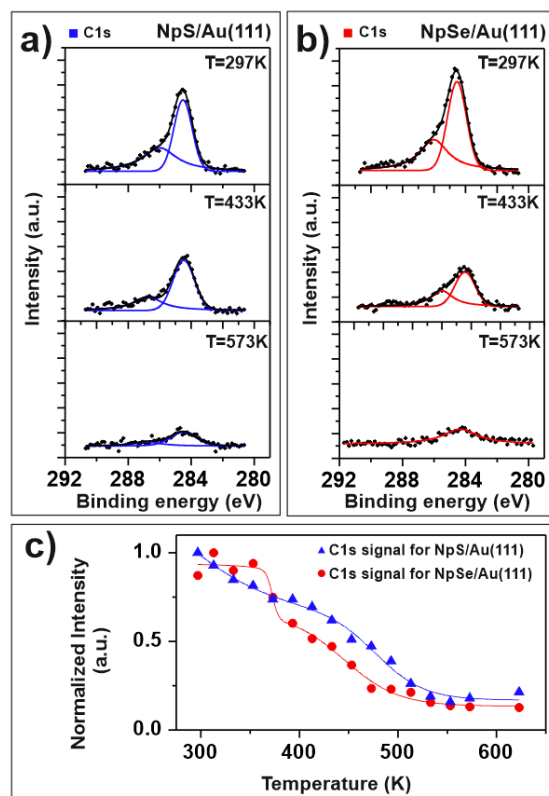
Figure 3. XPS data analysis. (a) and (b) show selected C 1s spectra obtained at different temperatures for NC-NapS/Au and NC-NapSe/Au, respectively (all spectra have the same vertical scale). (c) shows C 1s signal intensities normalized to the room-temperature values as a function of the sample temperature measured for NC-NapS/Au (blue points) and NC-NapSe/Au (red points). The color-coded lines in c are guides to the eye.
