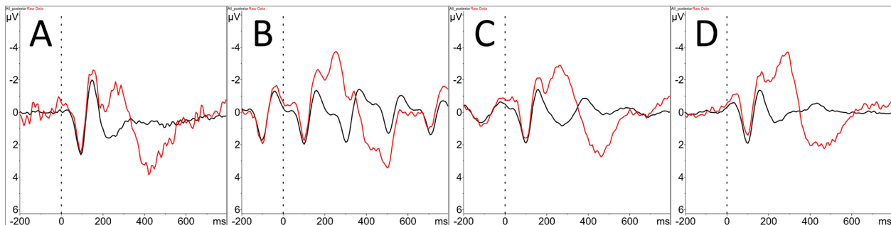
Figure 1. ERP waveforms averaged across target (red) and non-target (black) letter stimuli in four RSVP calibration conditions: [A] 1 Hz presentation with no stimulus jitter; [B] 5 Hz presentation with no jitter; [C] 5 Hz presentation with small jitter of \pm 50 ms; and [D] 5 Hz presentation with a large jitter of \pm 100 ms. Intrusion of the SSVEP signal is greatly decreased in conditions [C] and [D], compared to [B].
