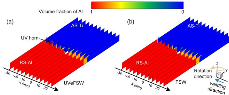
Fig. 11 Contour map of phase distribution along different cross-sections in the welding direction. (a) UVeFSW. (b) FSW
