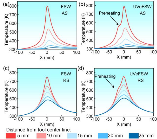
Fig. 9 Welding thermal cycle at different positions on the (a) AS of FSW, (b) AS of UVeFSW, (c) RS of FSW, (d) AS of UVeFSW
