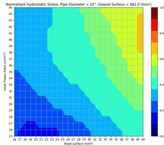
Fig. 11 Hydrostatic stress map as a function of the bead surface and the power ratio for a 10" diameter and a groove section of 462 mm 2 [8]
